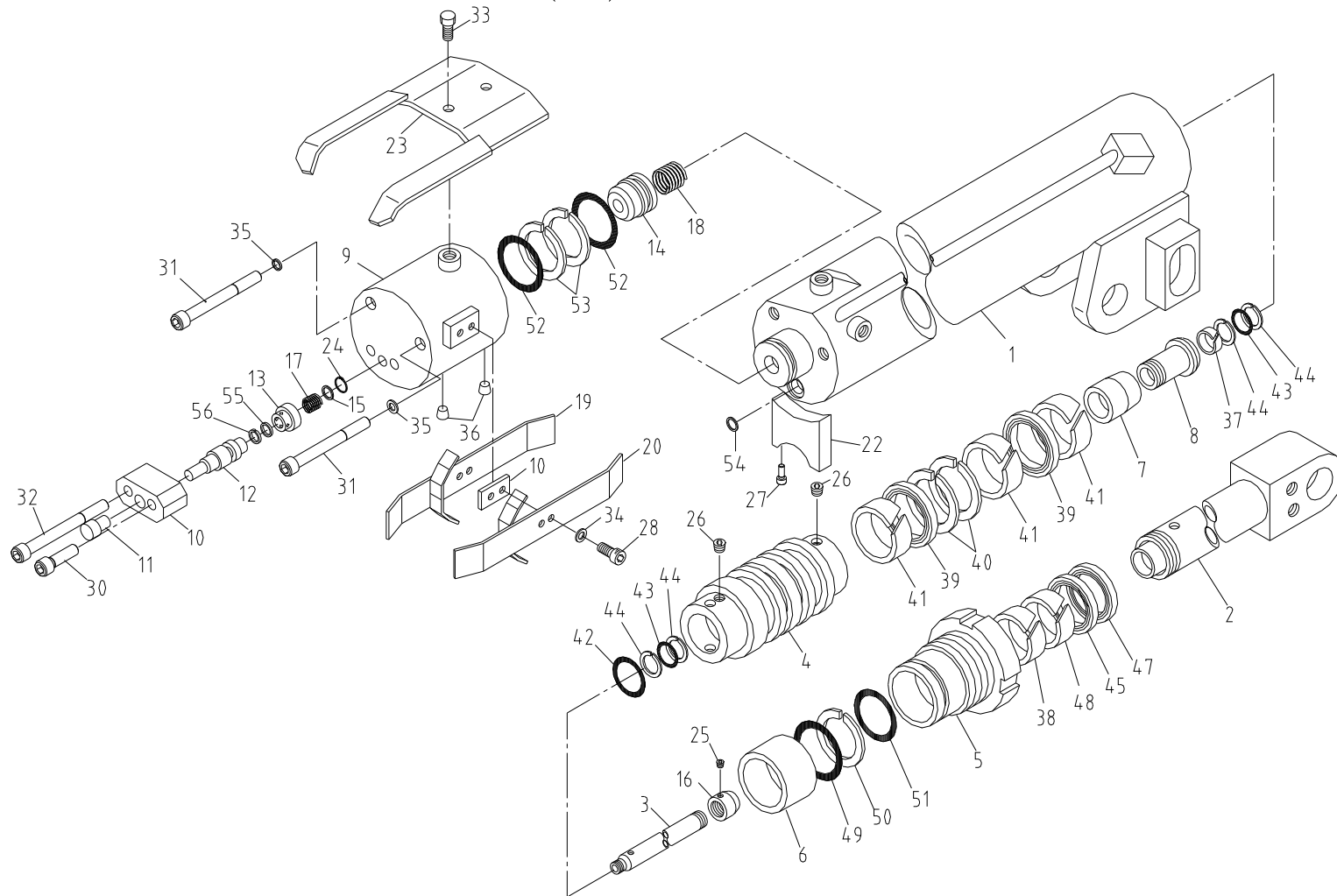
Fig. 1-1-1 SCS2016 TELESCOPIC CYL'(1st) ASS'Y
