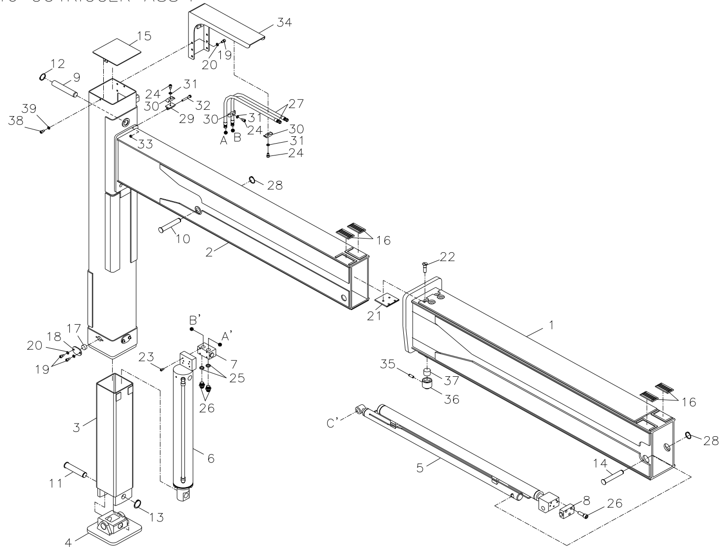
Fig. 4 SCS2016 OUTRIGGER ASS'Y
