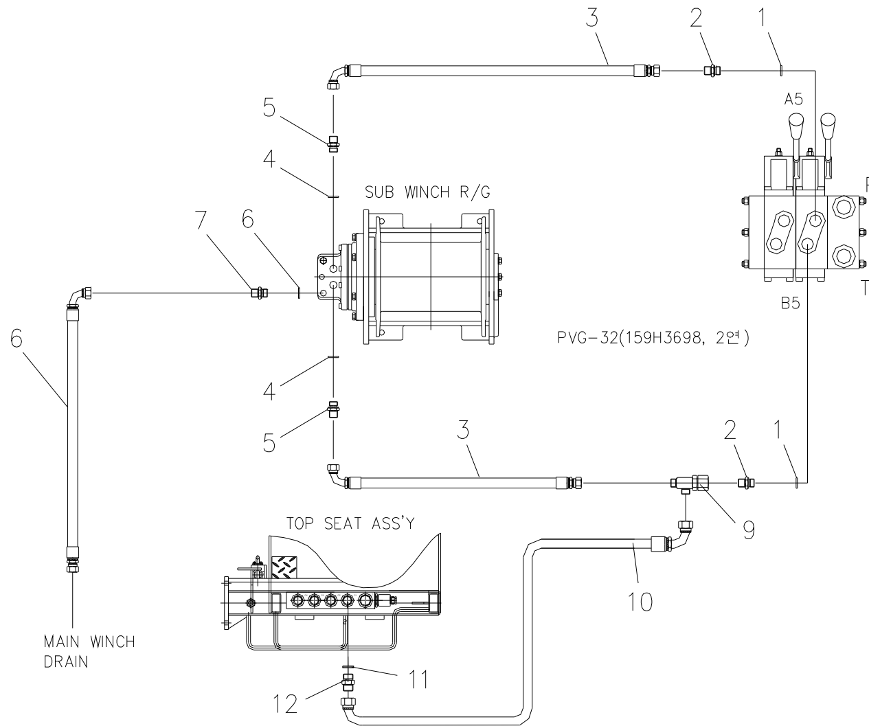
Fig. 12-1 SCS2016 SUB WINCH PIPING (F15 112)
