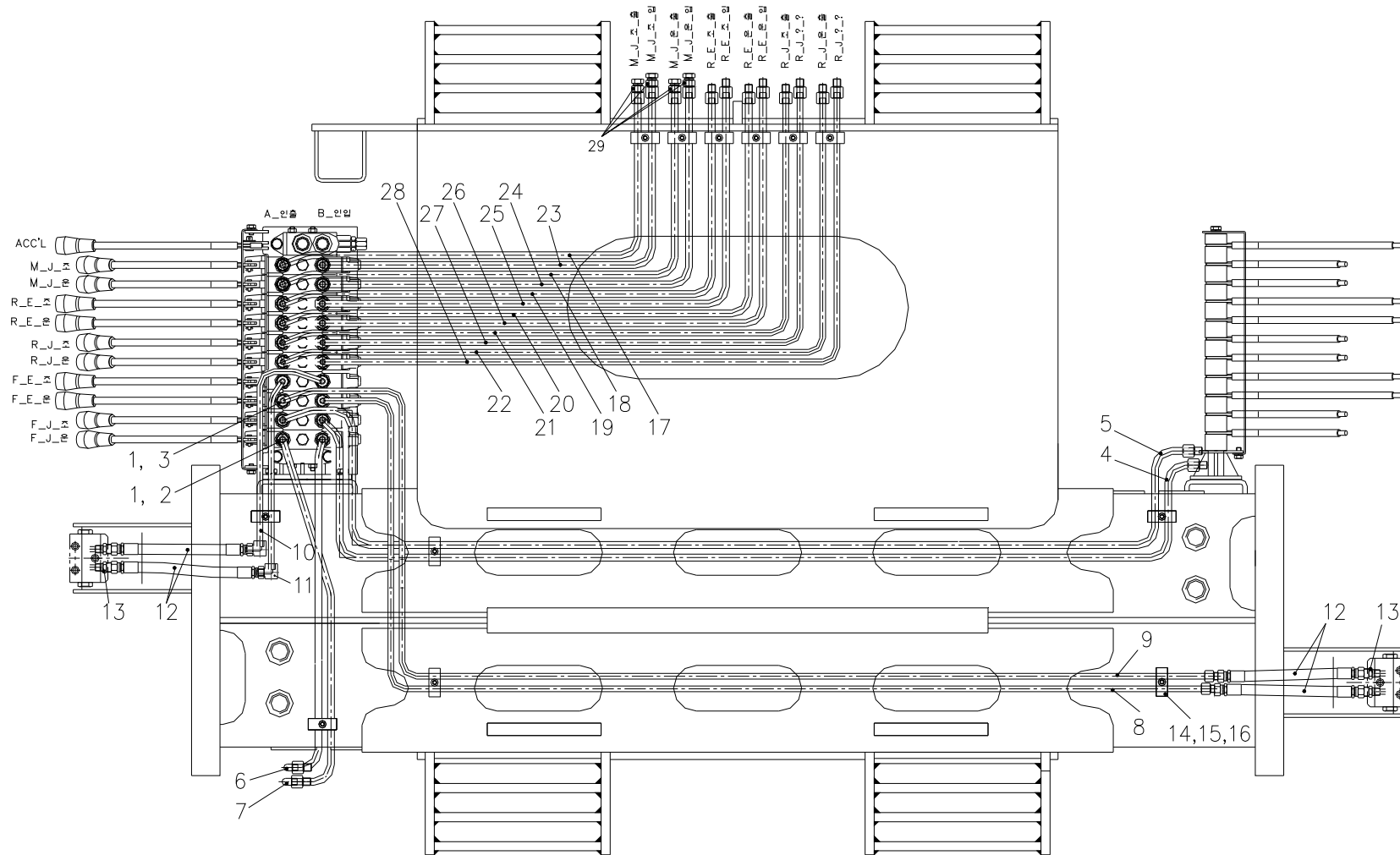
Fig. 5-7 SCS2016 OUTRIGGER PIPING
