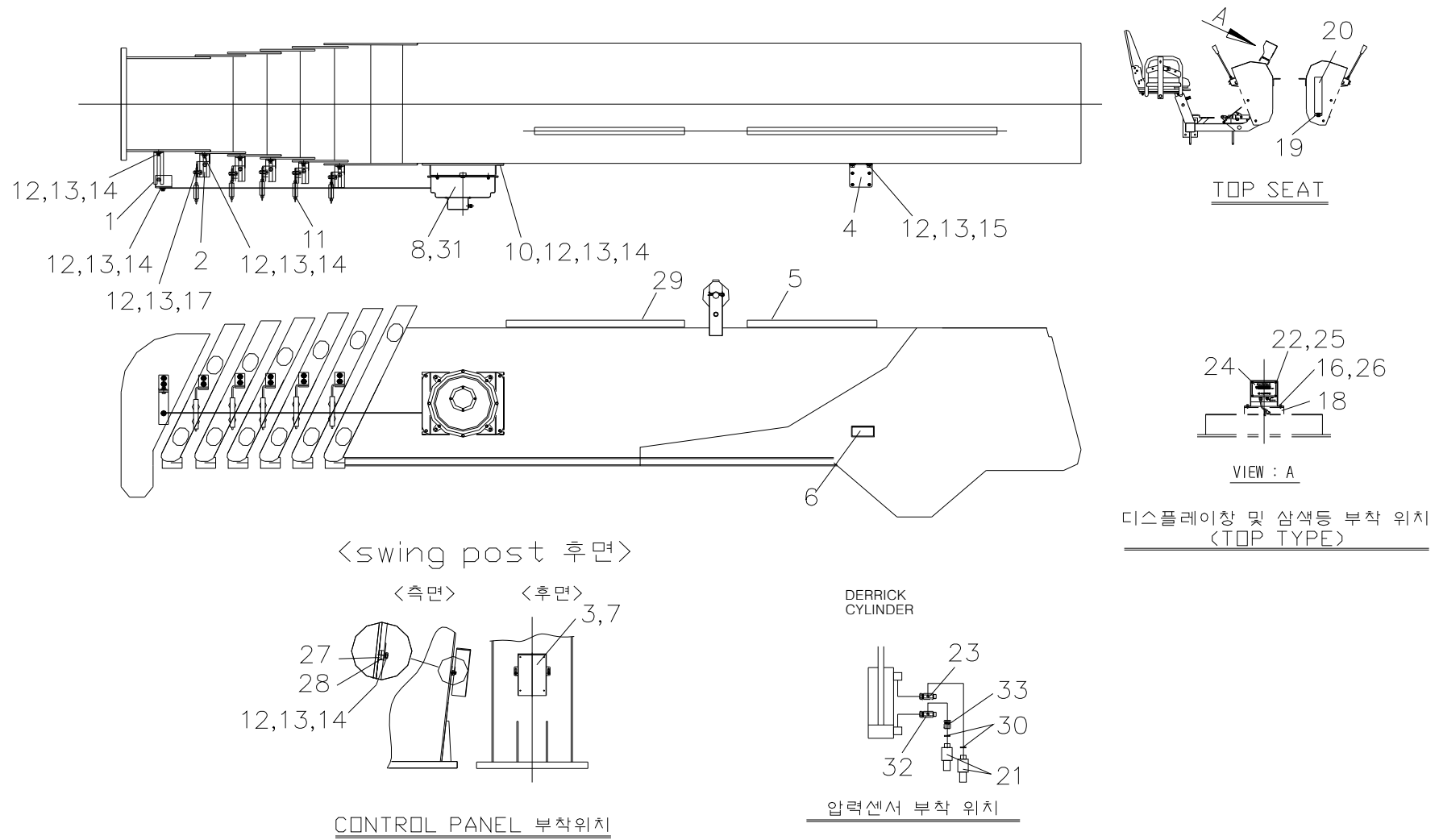
Fig. 17 SCS2016 AML ASS'Y
