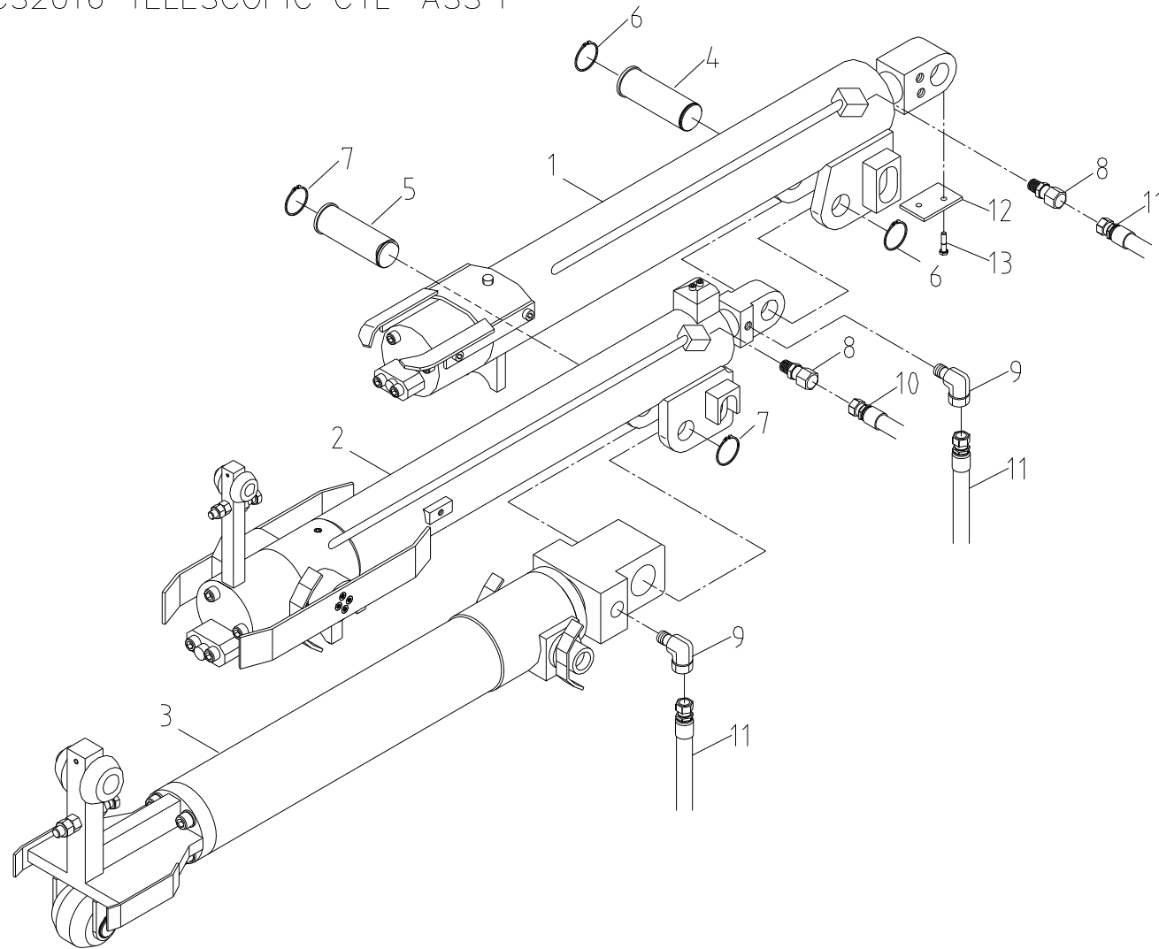
Fig. 1-1 SCS2016 TELESCOPIC CYL' ASS'Y
