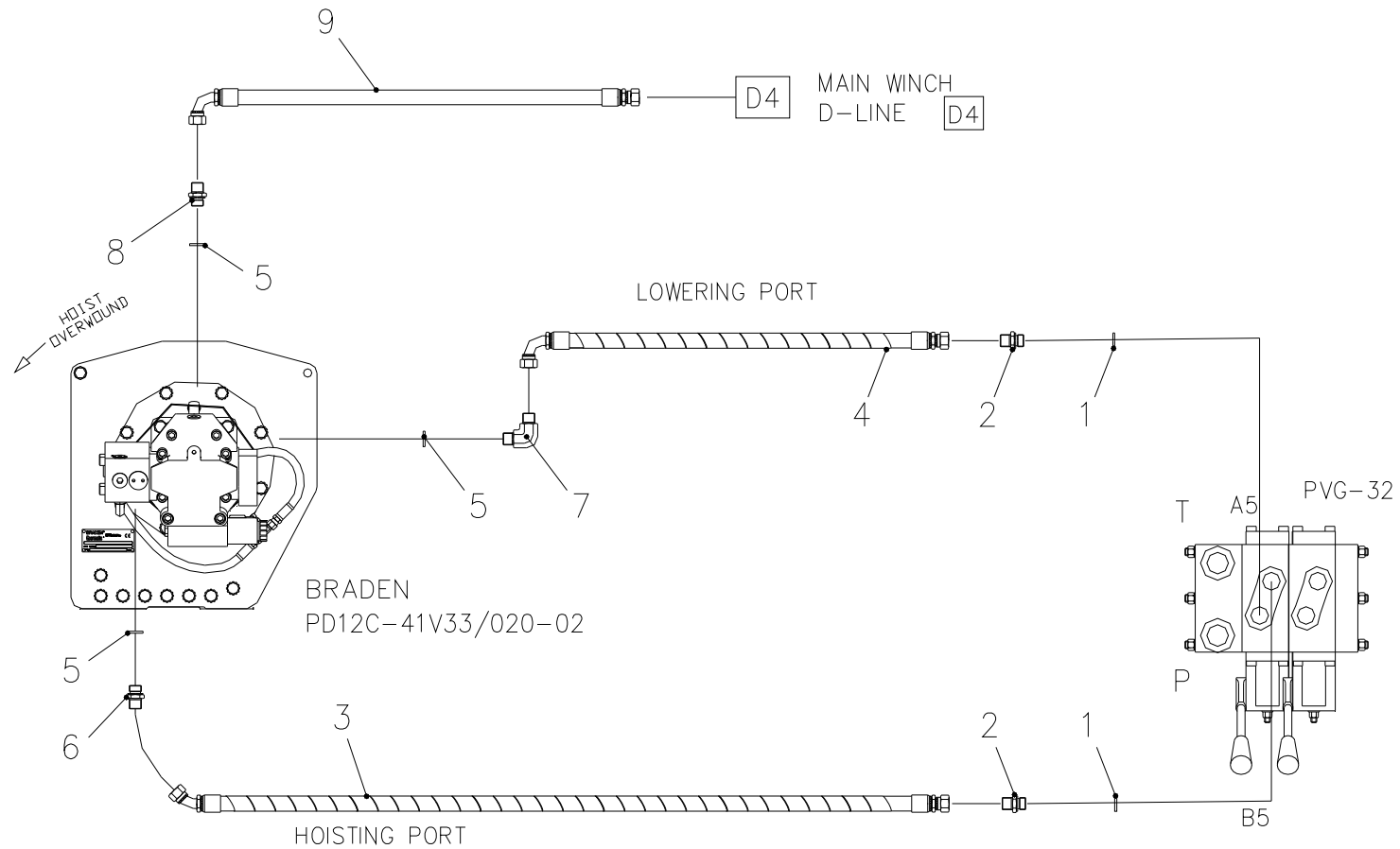
Fig. 12-1 SCS2016 SUB WINCH PIPING (W24 510)
